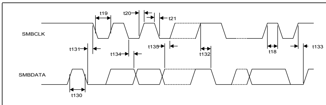
Figure 10-6. SMBus/SMLink Transaction
